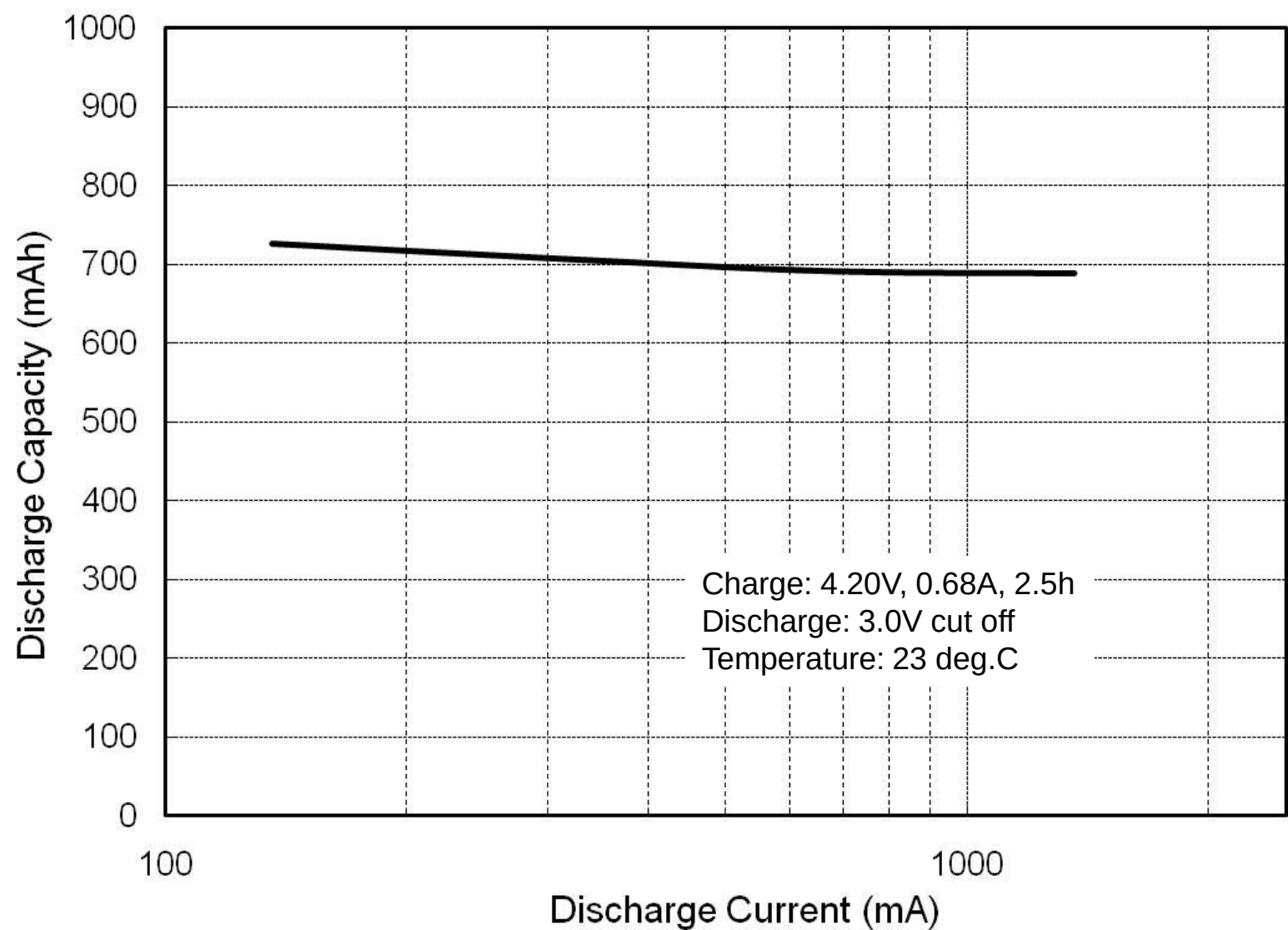
Discharge Load Characteristics (US14500VR2)
