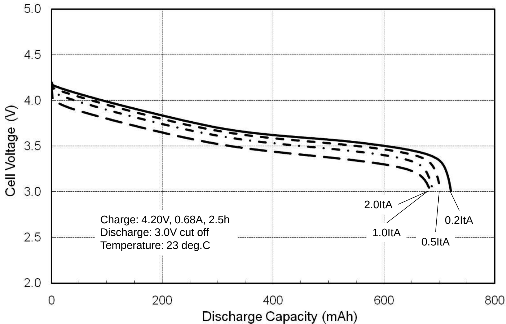
Discharge Load Characteristics (US14500VR2)
