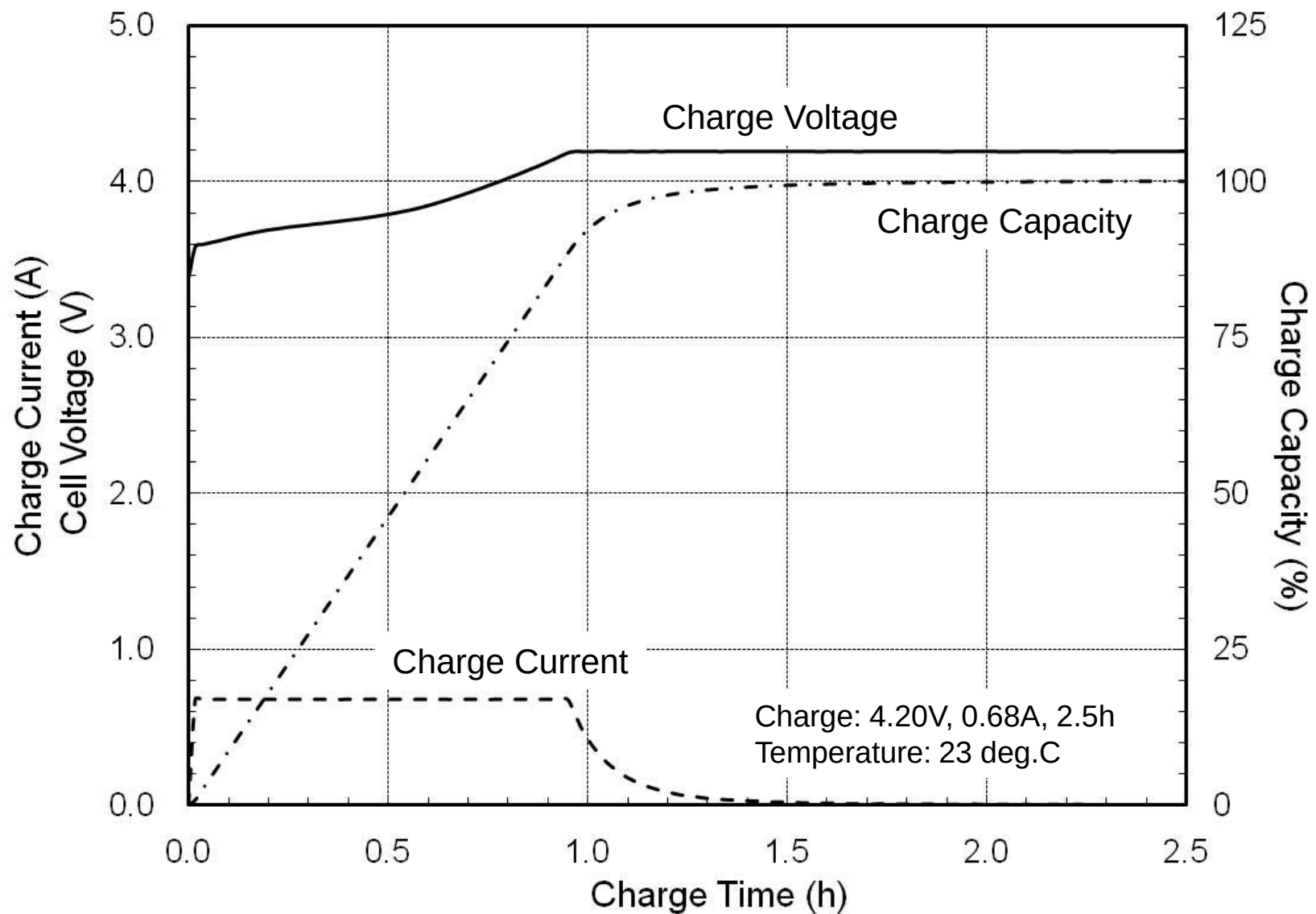
Charge Characteristics (US14500VR2)
