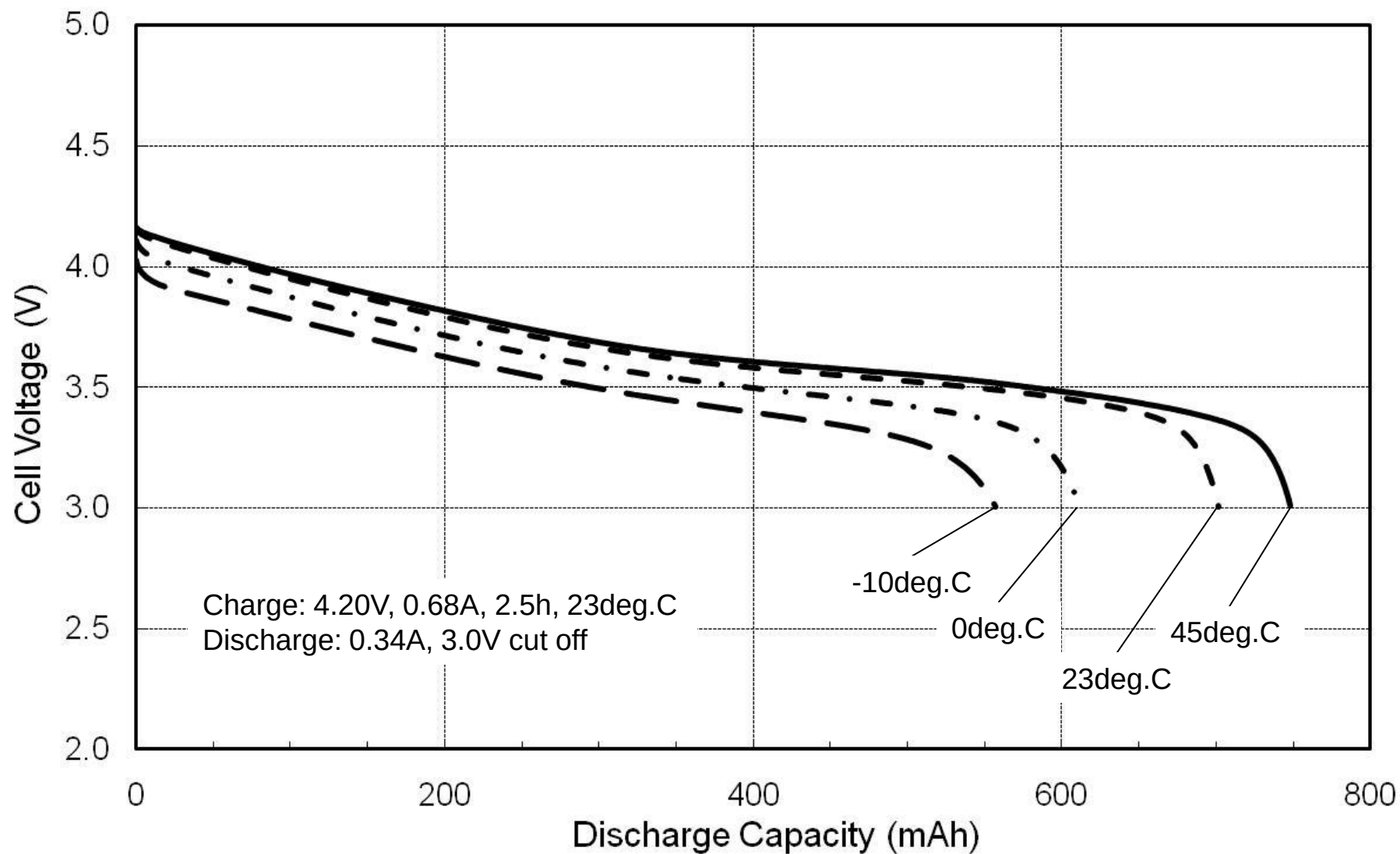
Temperature Dependence of Discharge Capacity (US14500VR2)
